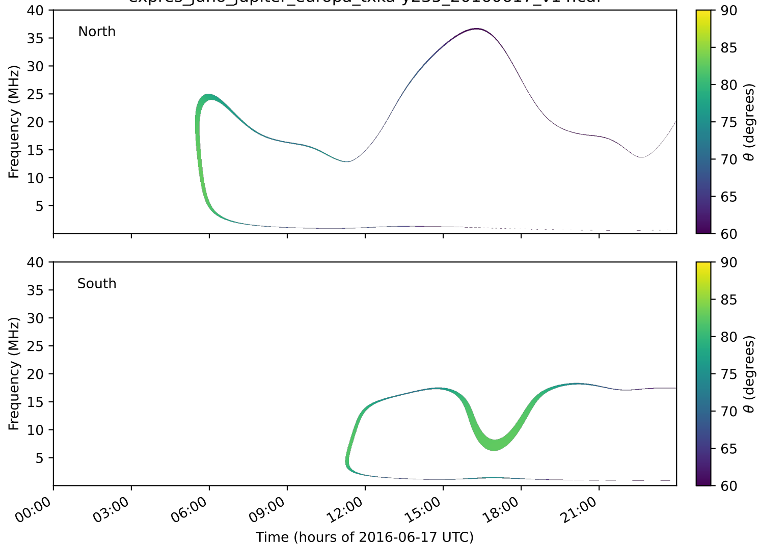
expres_juno_jupiter_europa_txka-y235_20160617_v14.cdf
