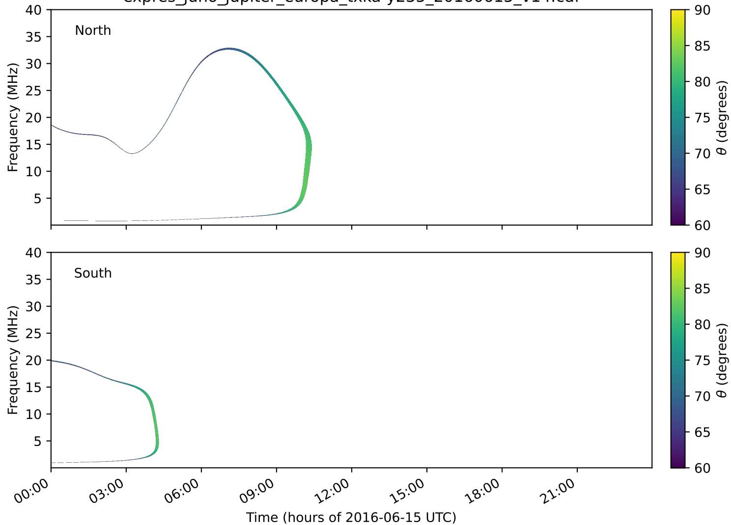
expres_juno_jupiter_europa_txka-y235_20160615_v14.cdf
