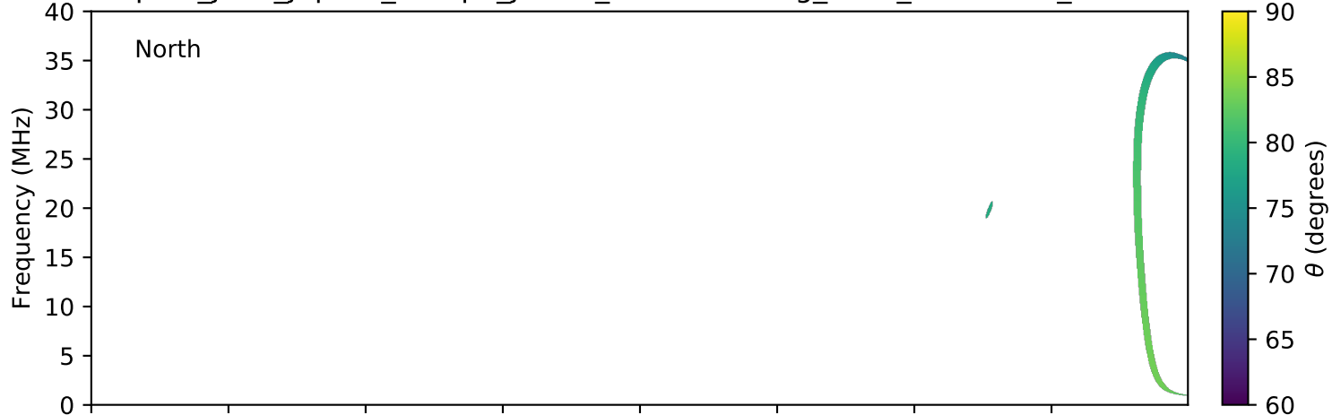
expres_juno_jupiter_europa_jrm09_lossc-wid1deg_3kev_20160627_v01.cdf
