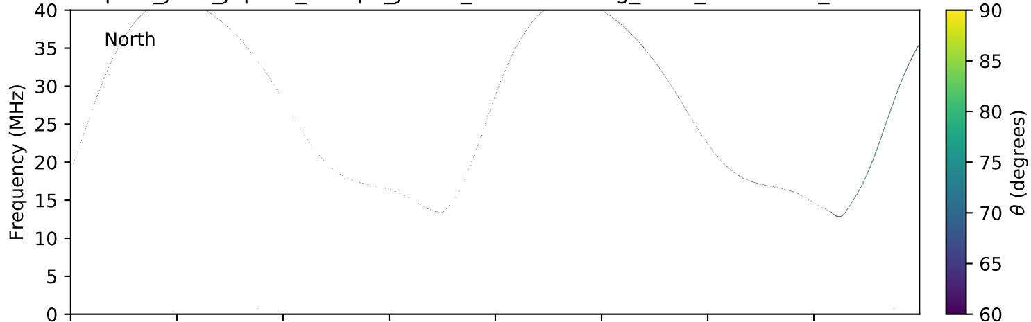
expres_juno_jupiter_europa_jrm09_lossc-wid1deg_3kev_20160625_v01.cdf
