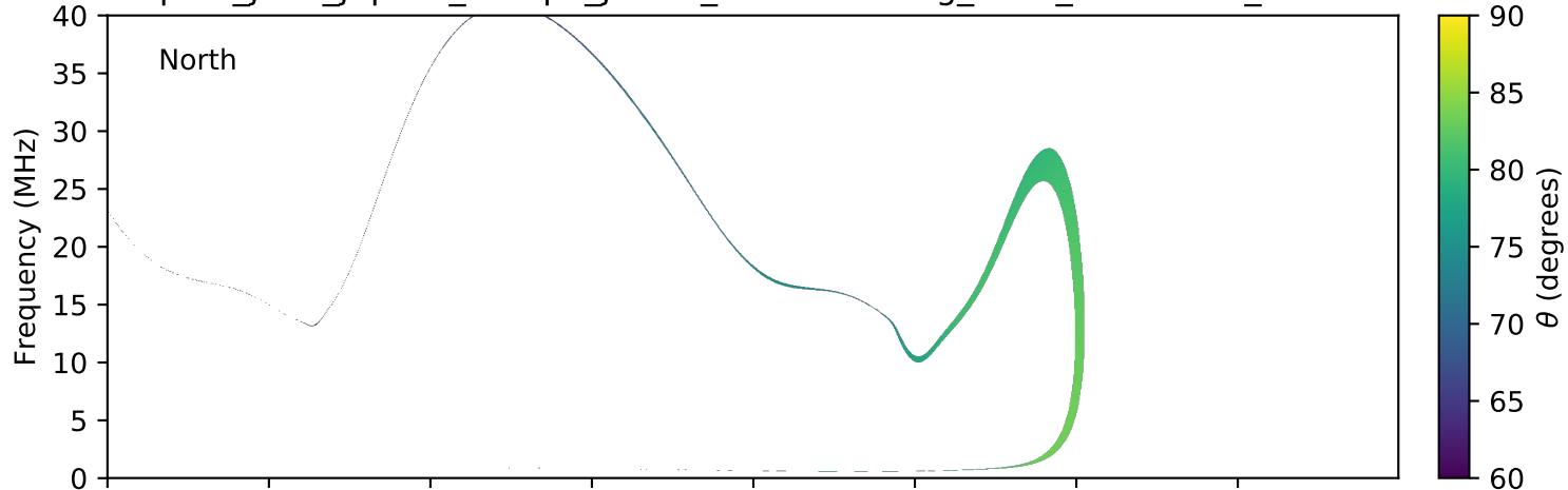
expres_juno_jupiter_europa_jrm09_lossc-wid1deg_3kev_20160622_v01.cdf
