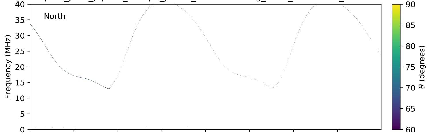
expres_juno_jupiter_europa_jrm09_lossc-wid1deg_3kev_20160621_v01.cdf
