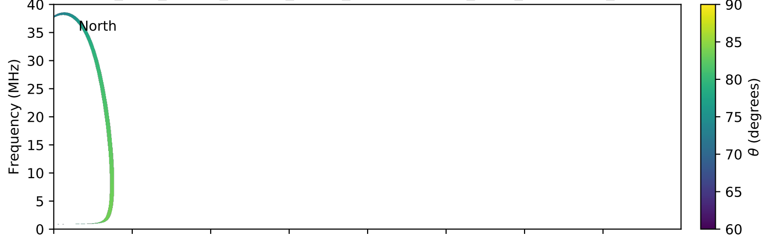
expres_juno_jupiter_europa_jrm09_lossc-wid1deg_3kev_20160619_v01.cdf
