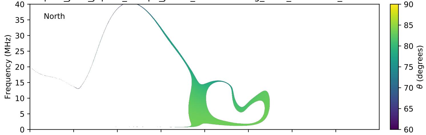
expres_juno_jupiter_europa_jrm09_lossc-wid1deg_3kev_20160615_v01.cdf
