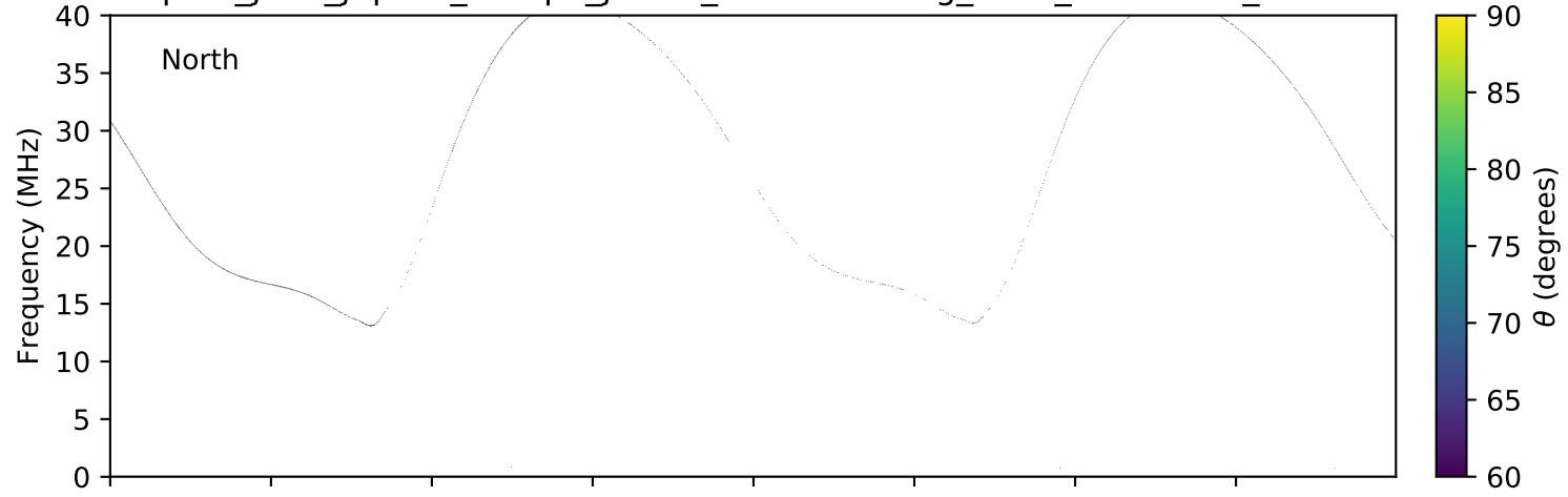
expres_juno_jupiter_europa_jrm09_lossc-wid1deg_3kev_20160614_v01.cdf
