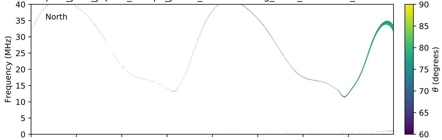
expres_juno_jupiter_europa_jrm09_lossc-wid1deg_3kev_20160611_v01.cdf
