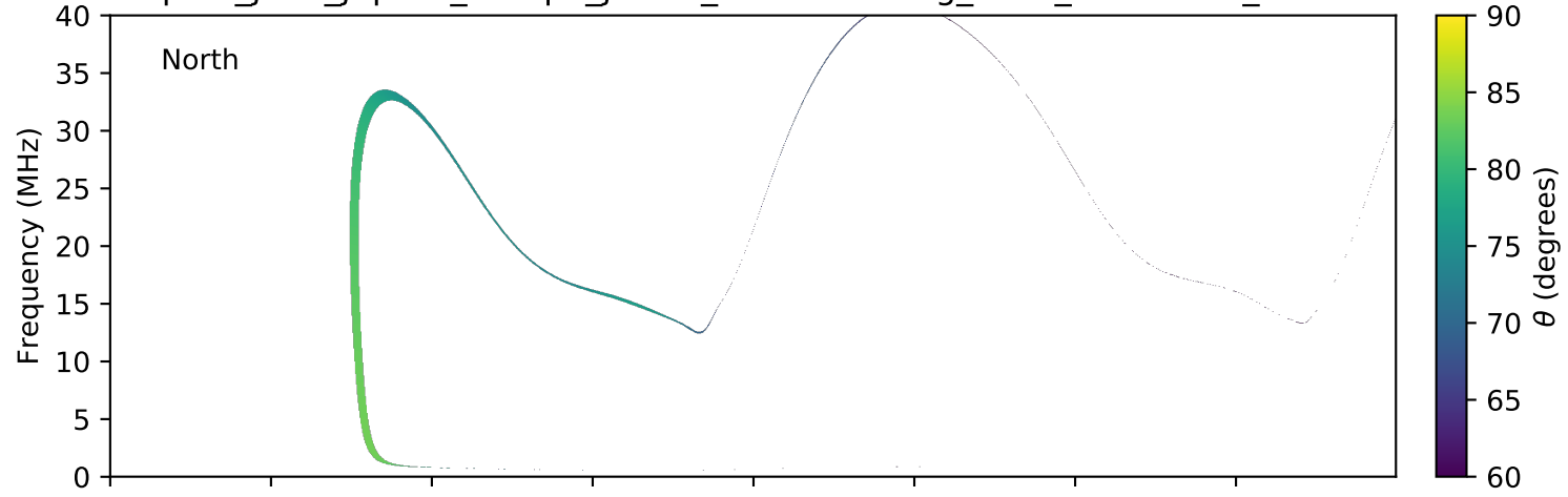
expres_juno_jupiter_europa_jrm09_lossc-wid1deg_3kev_20160610_v01.cdf
