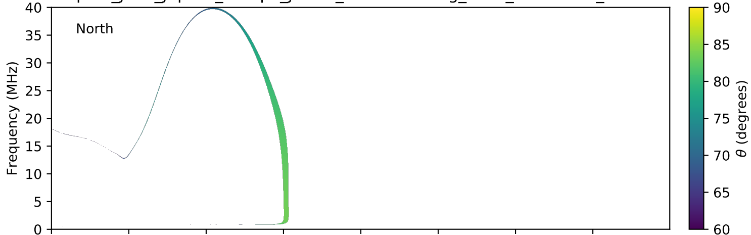
expres_juno_jupiter_europa_jrm09_lossc-wid1deg_3kev_20160608_v01.cdf
