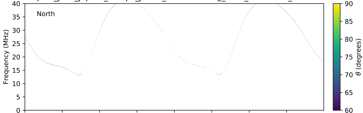
expres_juno_jupiter_europa_jrm09_lossc-wid1deg_3kev_20160607_v01.cdf
