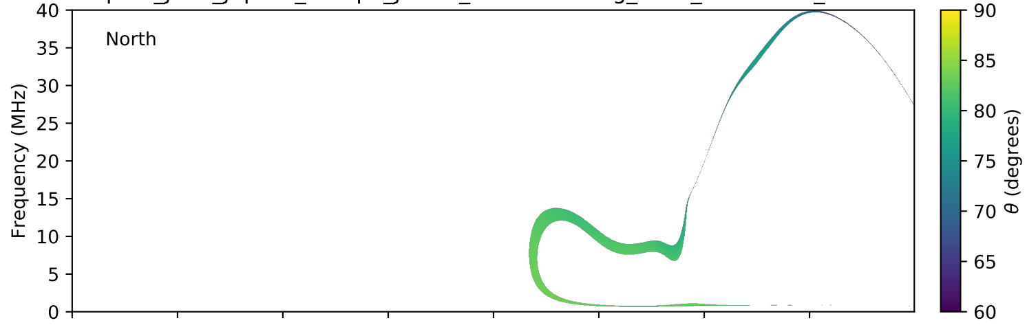
expres_juno_jupiter_europa_jrm09_lossc-wid1deg_3kev_20160606_v01.cdf
