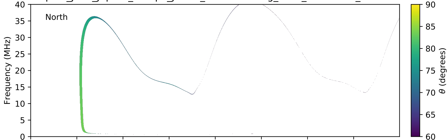
expres_juno_jupiter_europa_jrm09_lossc-wid1deg_3kev_20160603_v01.cdf
