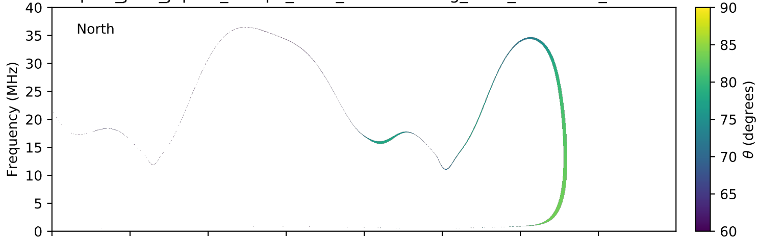
expres_juno_jupiter_europa_isaac_lossc-wid1deg_3kev_20160629_v01.cdf
