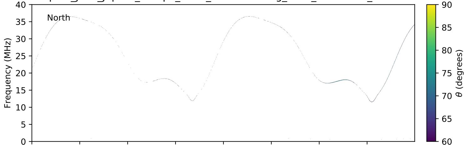
expres_juno_jupiter_europa_isaac_lossc-wid1deg_3kev_20160625_v01.cdf
