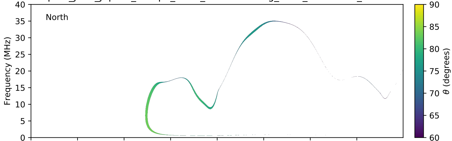
expres_juno_jupiter_europa_isaac_lossc-wid1deg_3kev_20160624_v01.cdf
