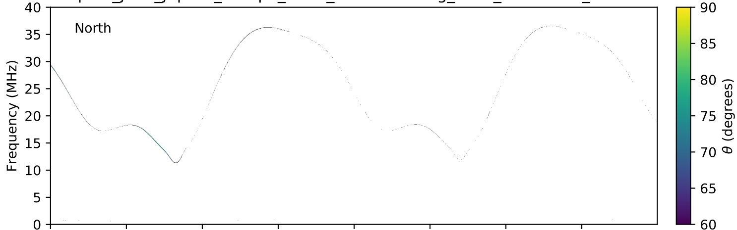
expres_juno_jupiter_europa_isaac_lossc-wid1deg_3kev_20160621_v01.cdf
