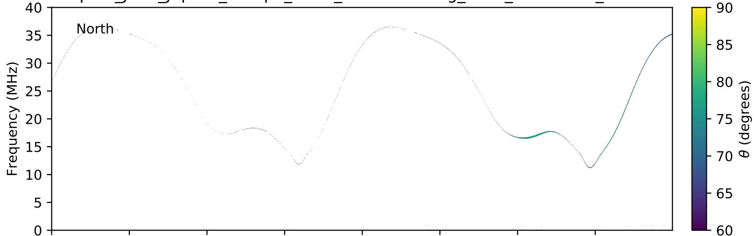
expres_juno_jupiter_europa_isaac_lossc-wid1deg_3kev_20160618_v01.cdf
