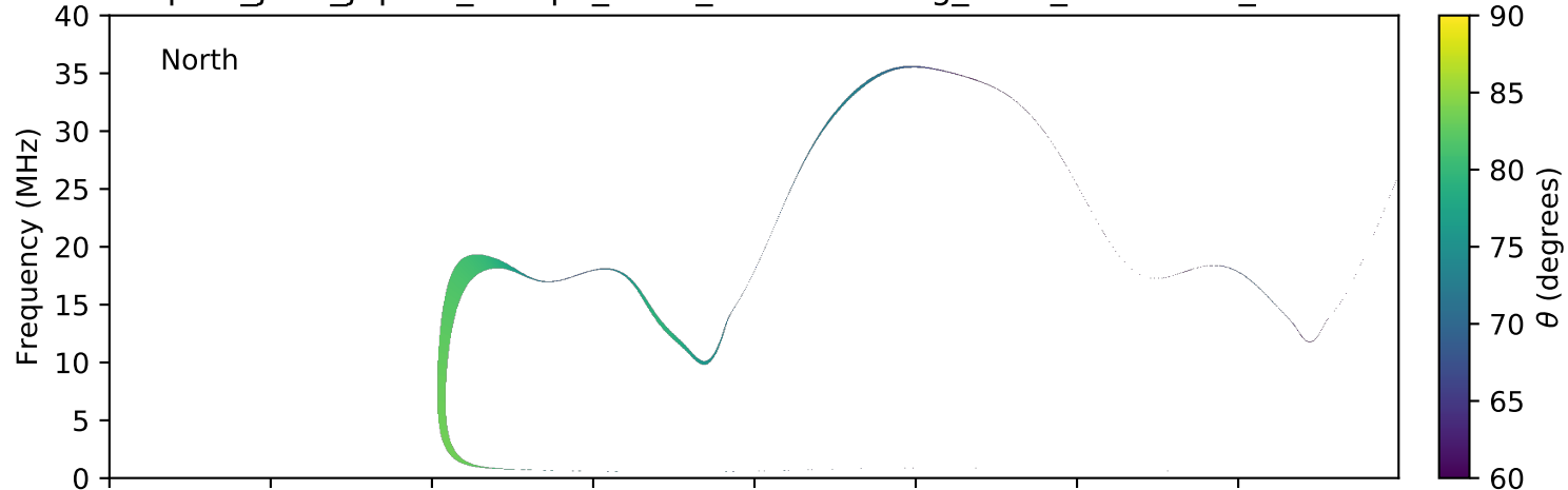
expres_juno_jupiter_europa_isaac_lossc-wid1deg_3kev_20160617_v01.cdf
