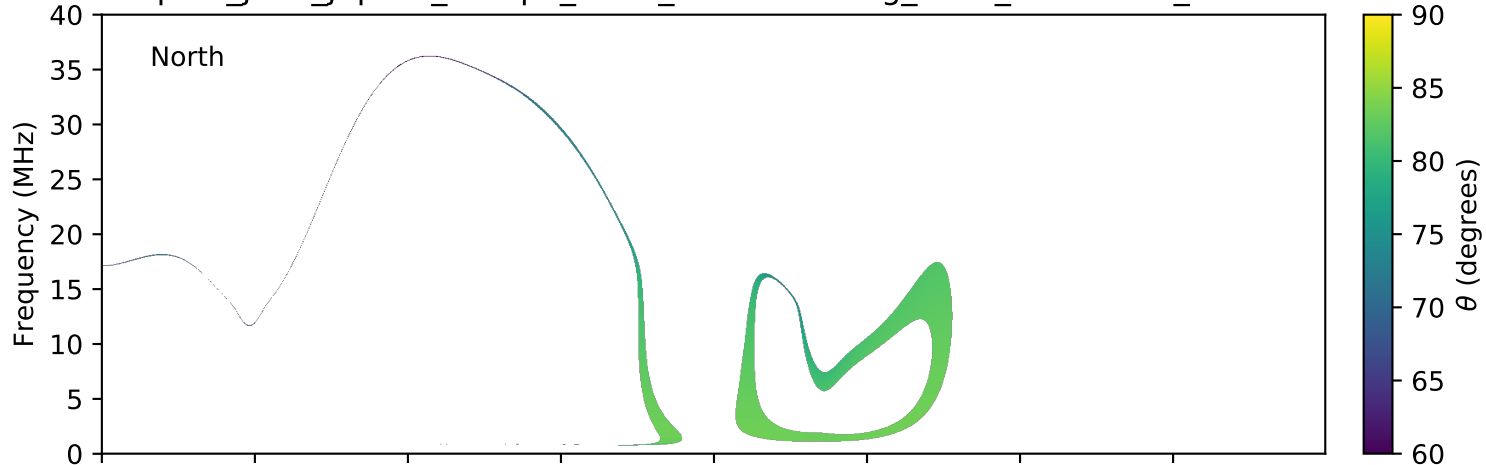
expres_juno_jupiter_europa_isaac_lossc-wid1deg_3kev_20160615_v01.cdf
