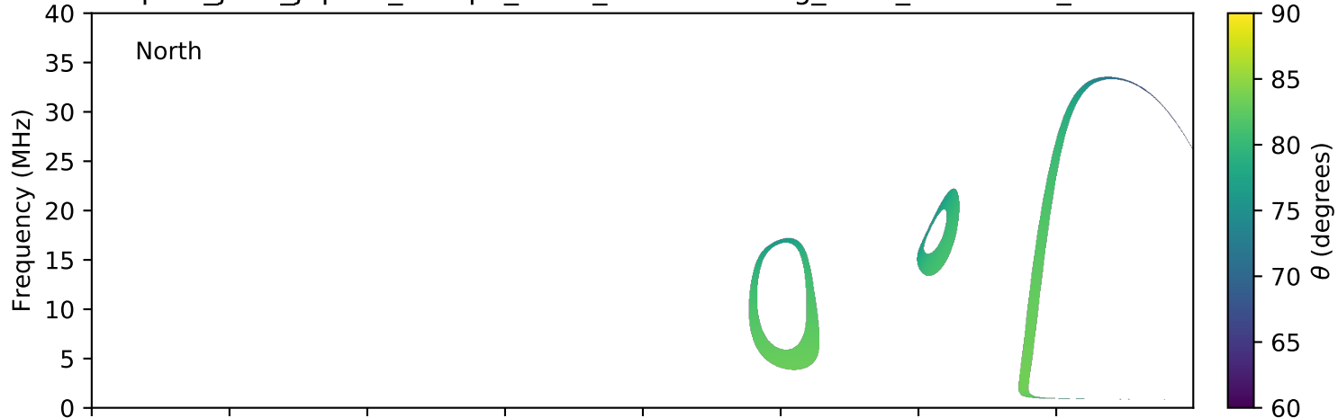
expres_juno_jupiter_europa_isaac_lossc-wid1deg_3kev_20160613_v01.cdf
