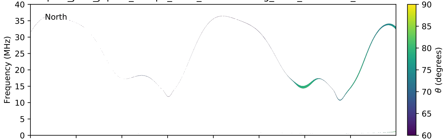
expres_juno_jupiter_europa_isaac_lossc-wid1deg_3kev_20160611_v01.cdf
