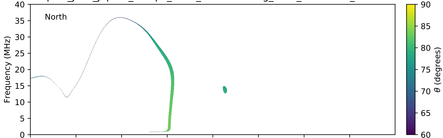
expres_juno_jupiter_europa_isaac_lossc-wid1deg_3kev_20160608_v01.cdf
