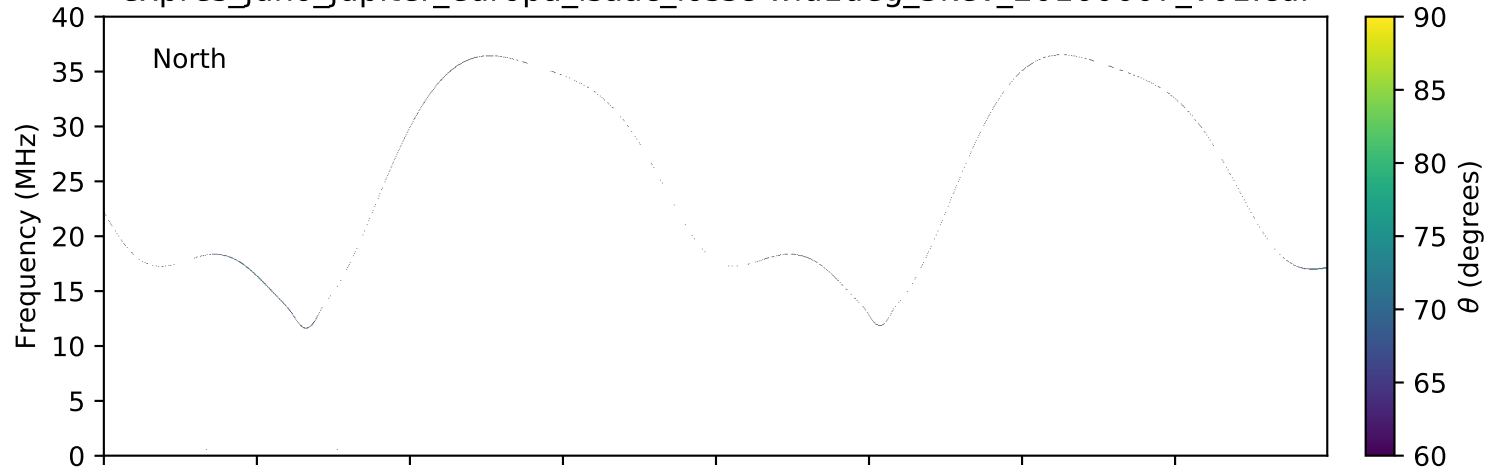
expres_juno_jupiter_europa_isaac_lossc-wid1deg_3kev_20160607_v01.cdf
