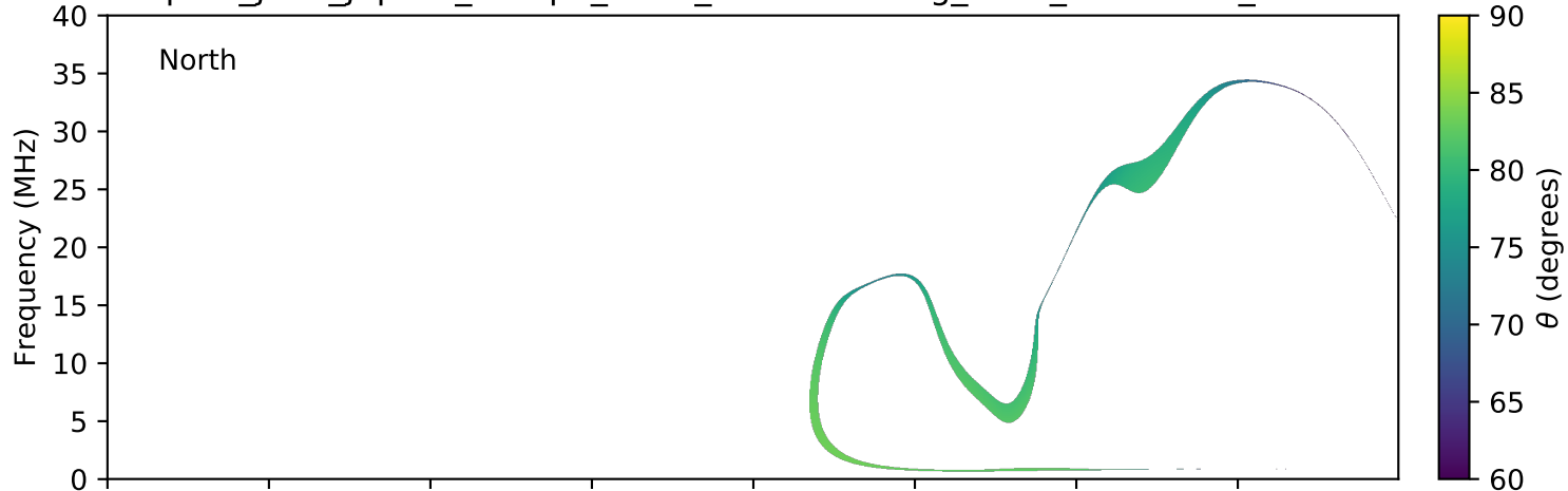
expres_juno_jupiter_europa_isaac_lossc-wid1deg_3kev_20160606_v01.cdf
