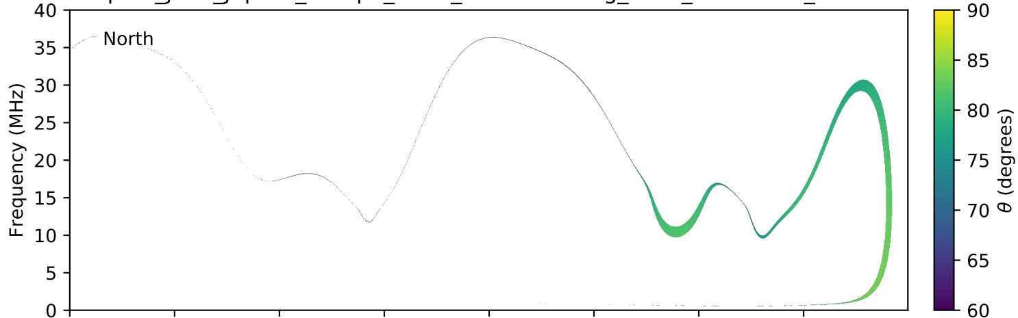
expres_juno_jupiter_europa_isaac_lossc-wid1deg_3kev_20160604_v01.cdf
