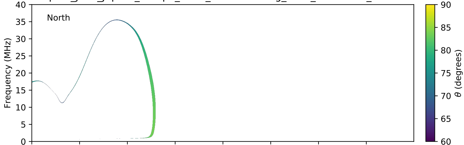
expres_juno_jupiter_europa_isaac_lossc-wid1deg_3kev_20160601_v01.cdf
