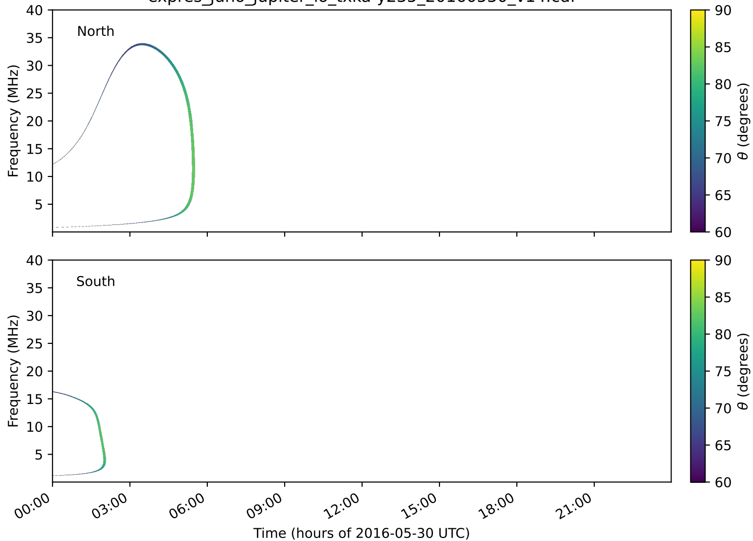
expres_juno_jupiter_io_txka-y235_20160530_v14.cdf
