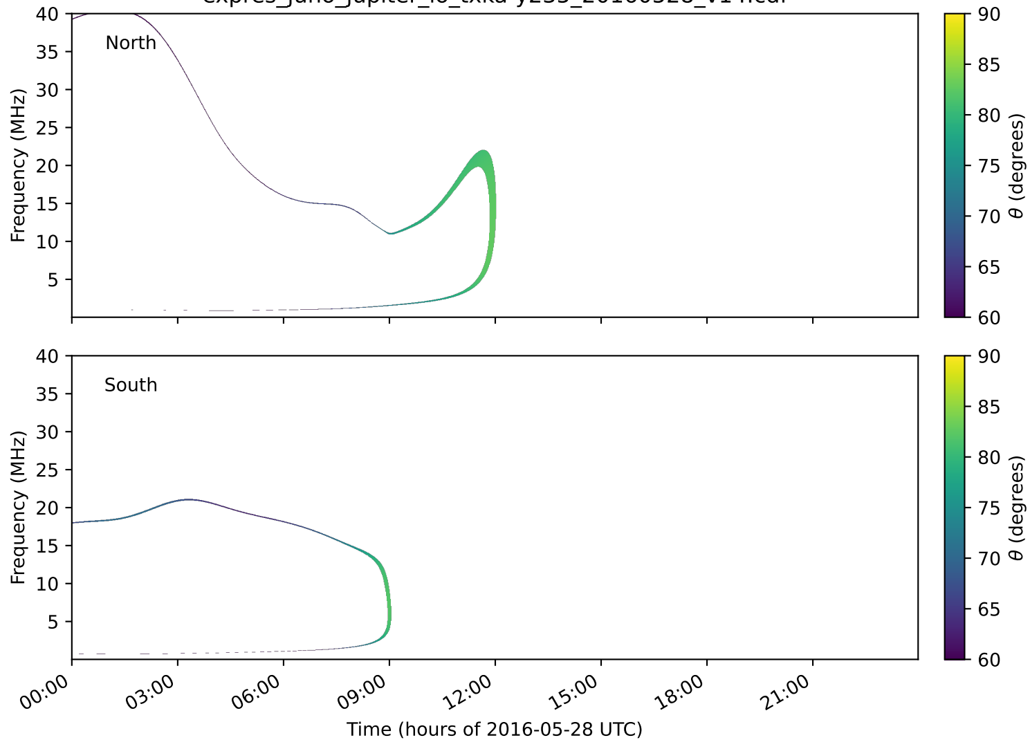
expres_juno_jupiter_io_txka-y235_20160528_v14.cdf
