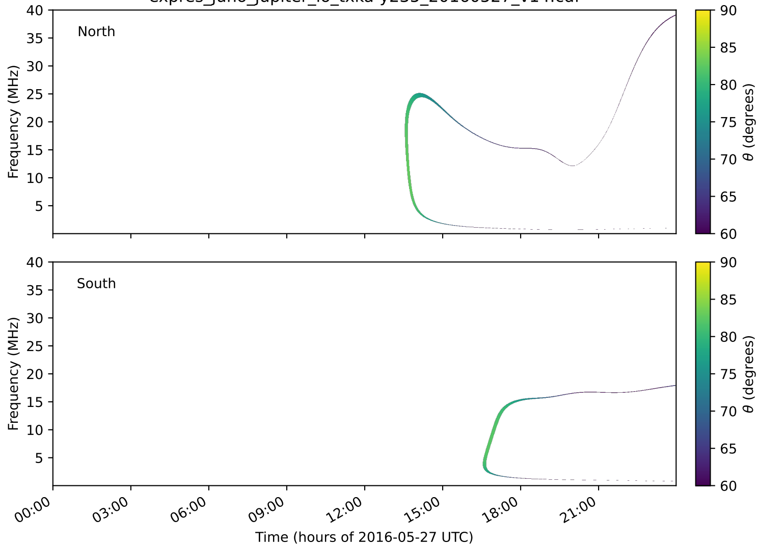
expres_juno_jupiter_io_txka-y235_20160527_v14.cdf
