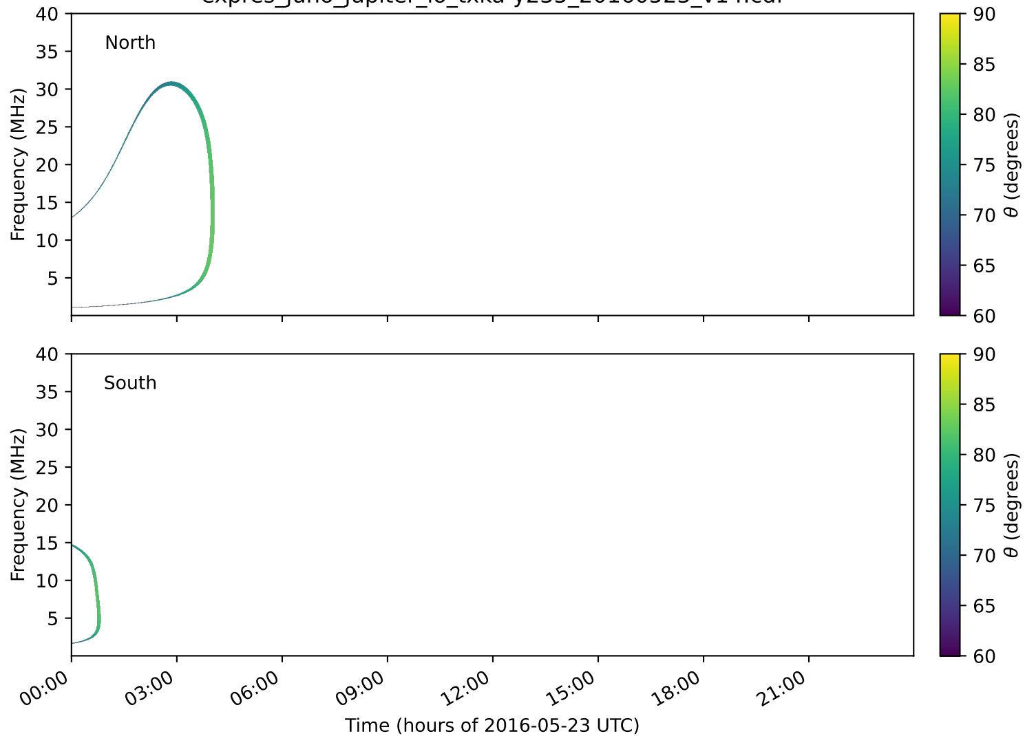
expres_juno_jupiter_io_txka-y235_20160523_v14.cdf
