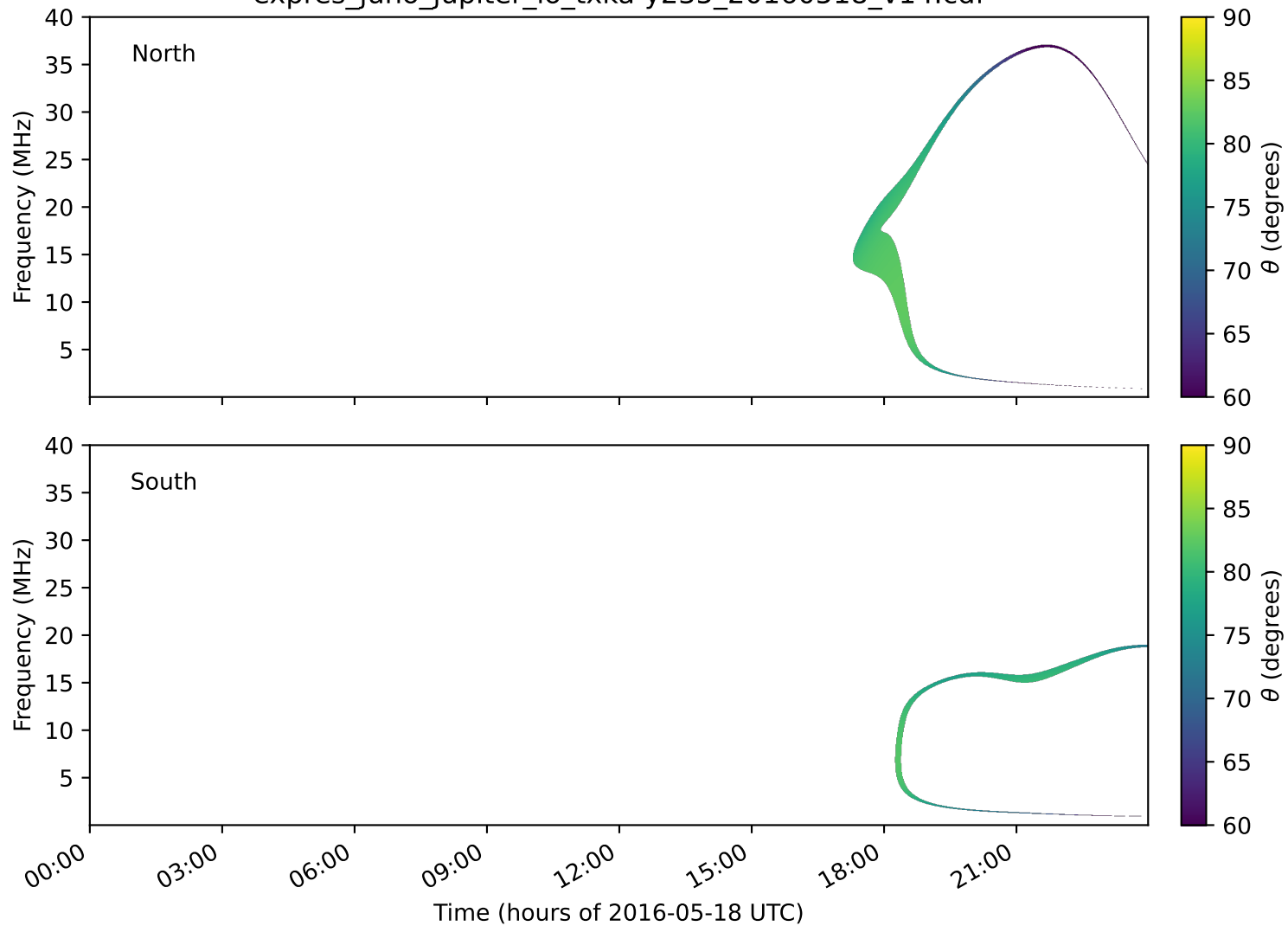
expres_juno_jupiter_io_txka-y235_20160518_v14.cdf
