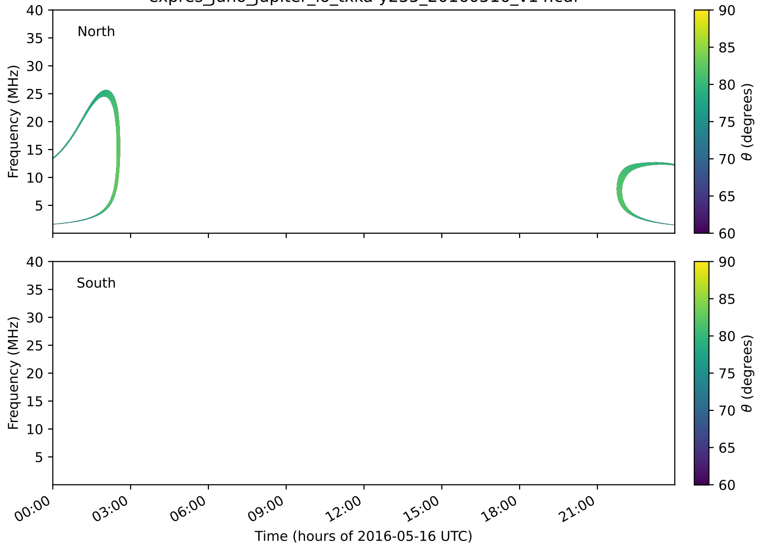
expres_juno_jupiter_io_txka-y235_20160516_v14.cdf
