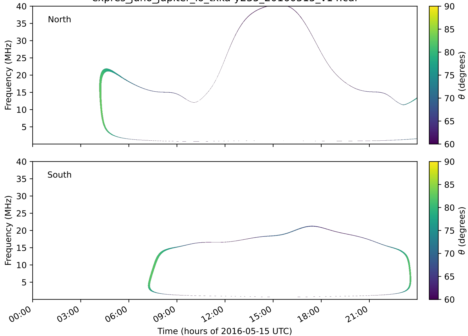
expres_juno_jupiter_io_txka-y235_20160515_v14.cdf
