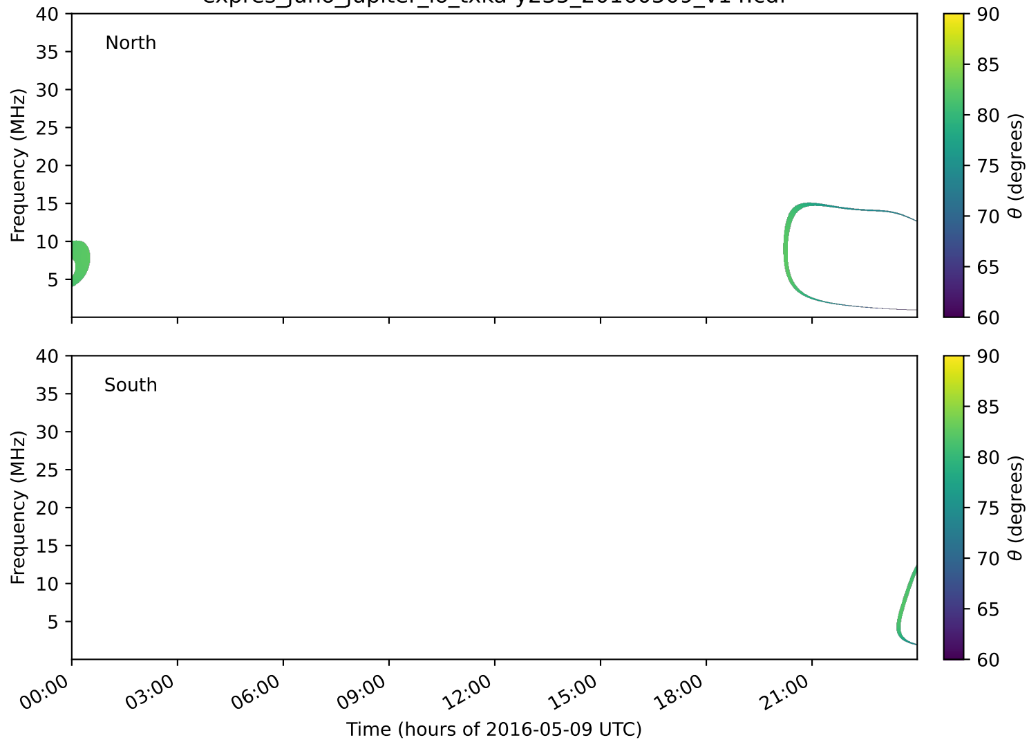
expres_juno_jupiter_io_txka-y235_20160509_v14.cdf
