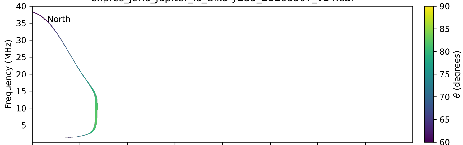
expres_juno_jupiter_io_txka-y235_20160507_v14.cdf
