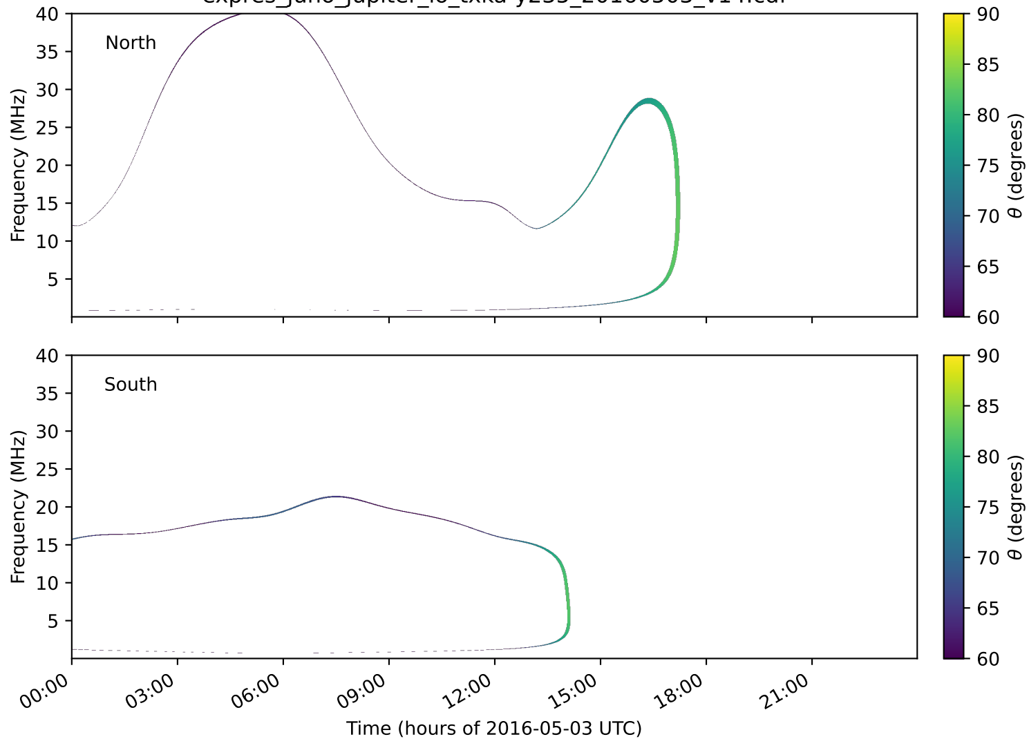
expres_juno_jupiter_io_txka-y235_20160503_v14.cdf
