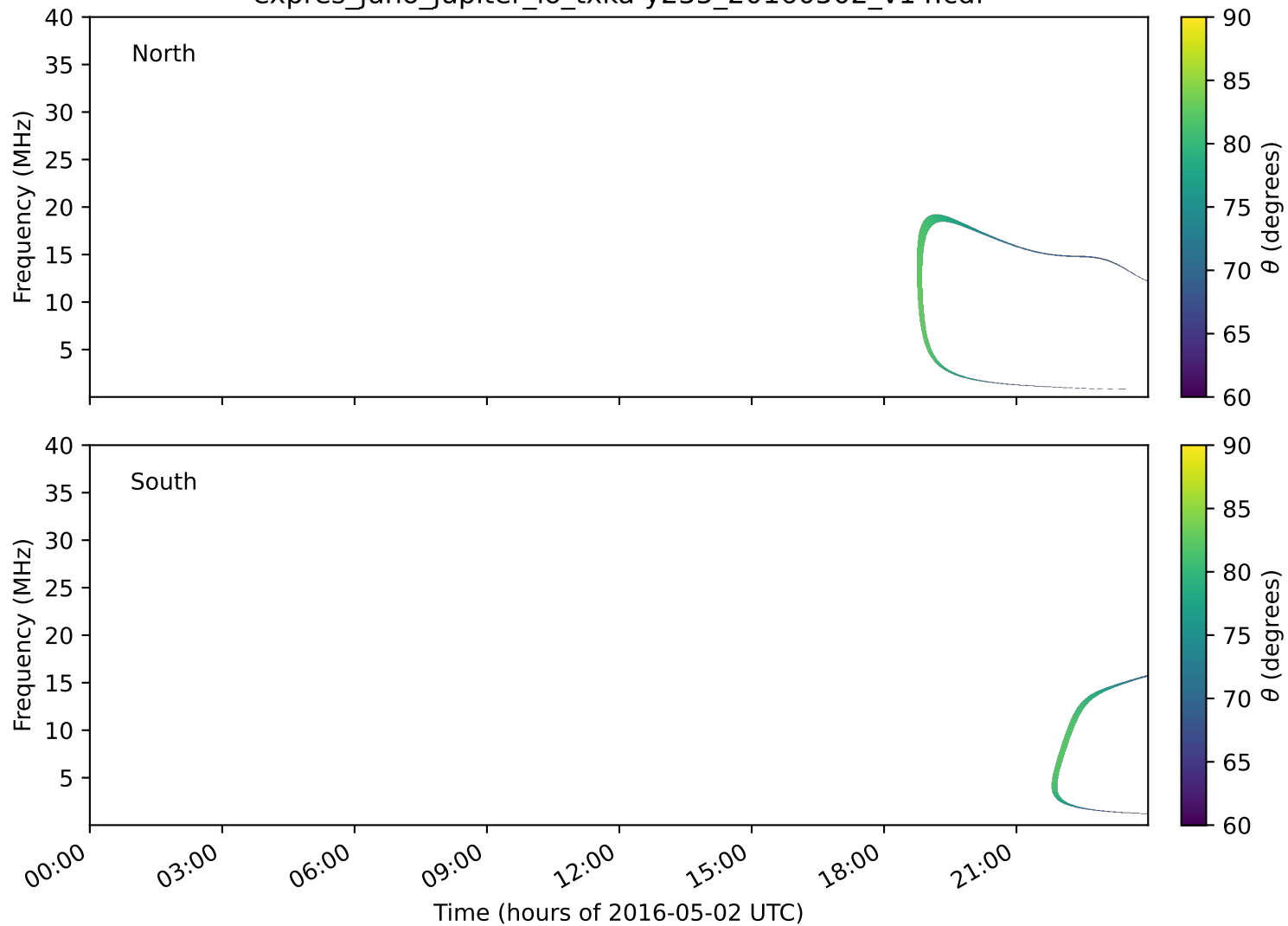
expres_juno_jupiter_io_txka-y235_20160502_v14.cdf
