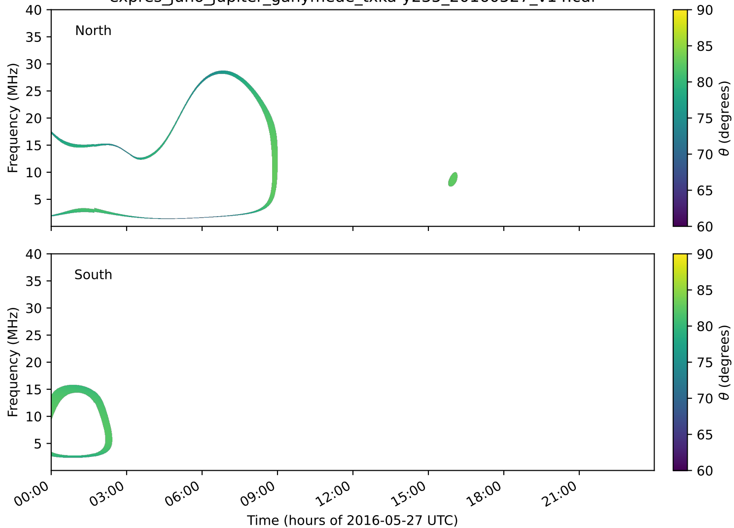
expres_juno_jupiter_ganymede_txka-y235_20160527_v14.cdf
