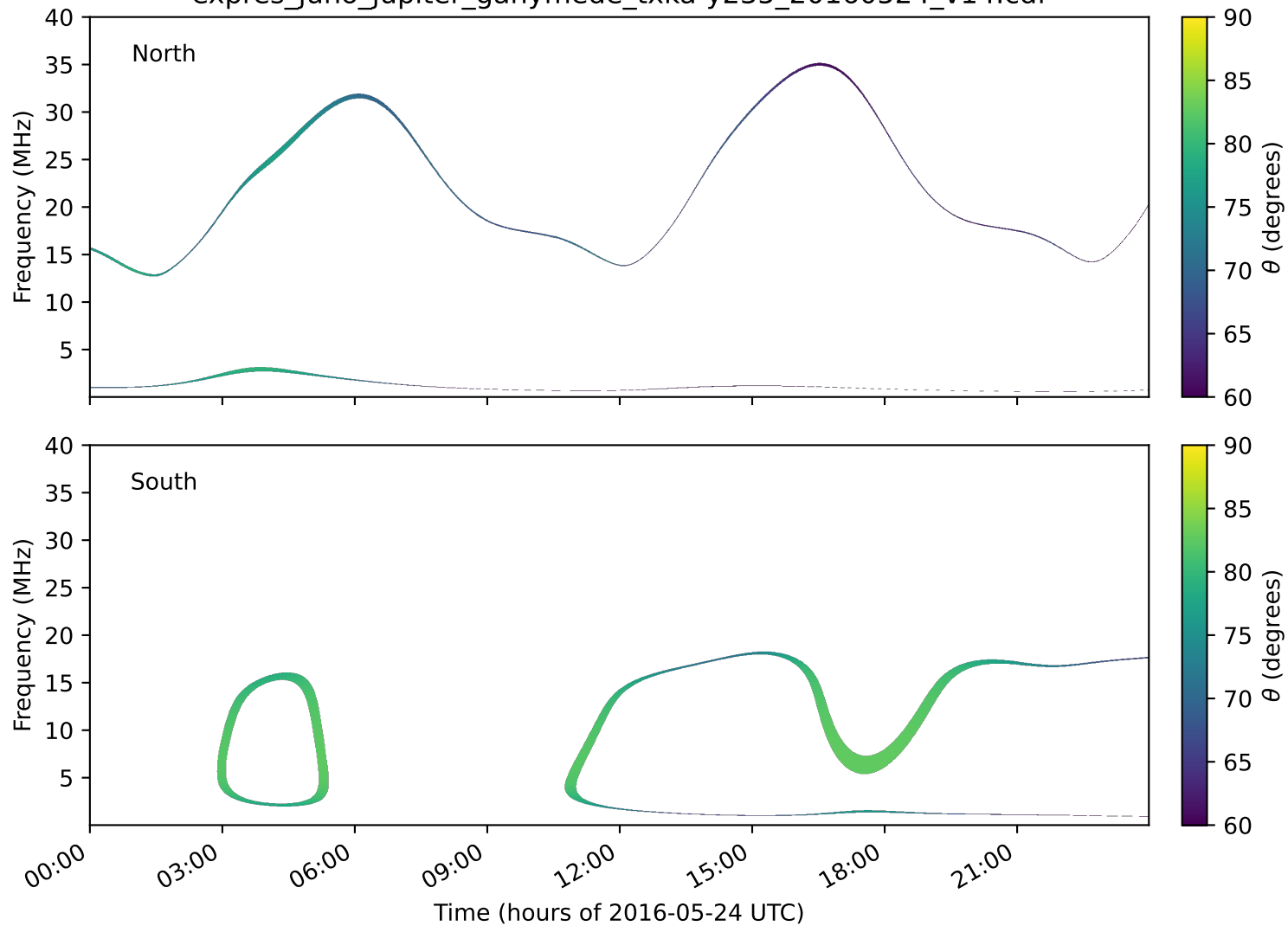
expres_juno_jupiter_ganymede_txka-y235_20160524_v14.cdf
