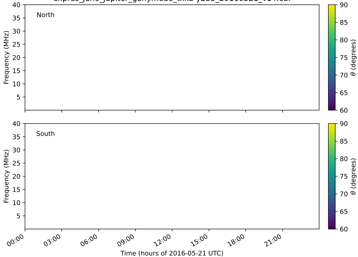
expres_juno_jupiter_ganymede_txka-y235_20160521_v14.cdf
