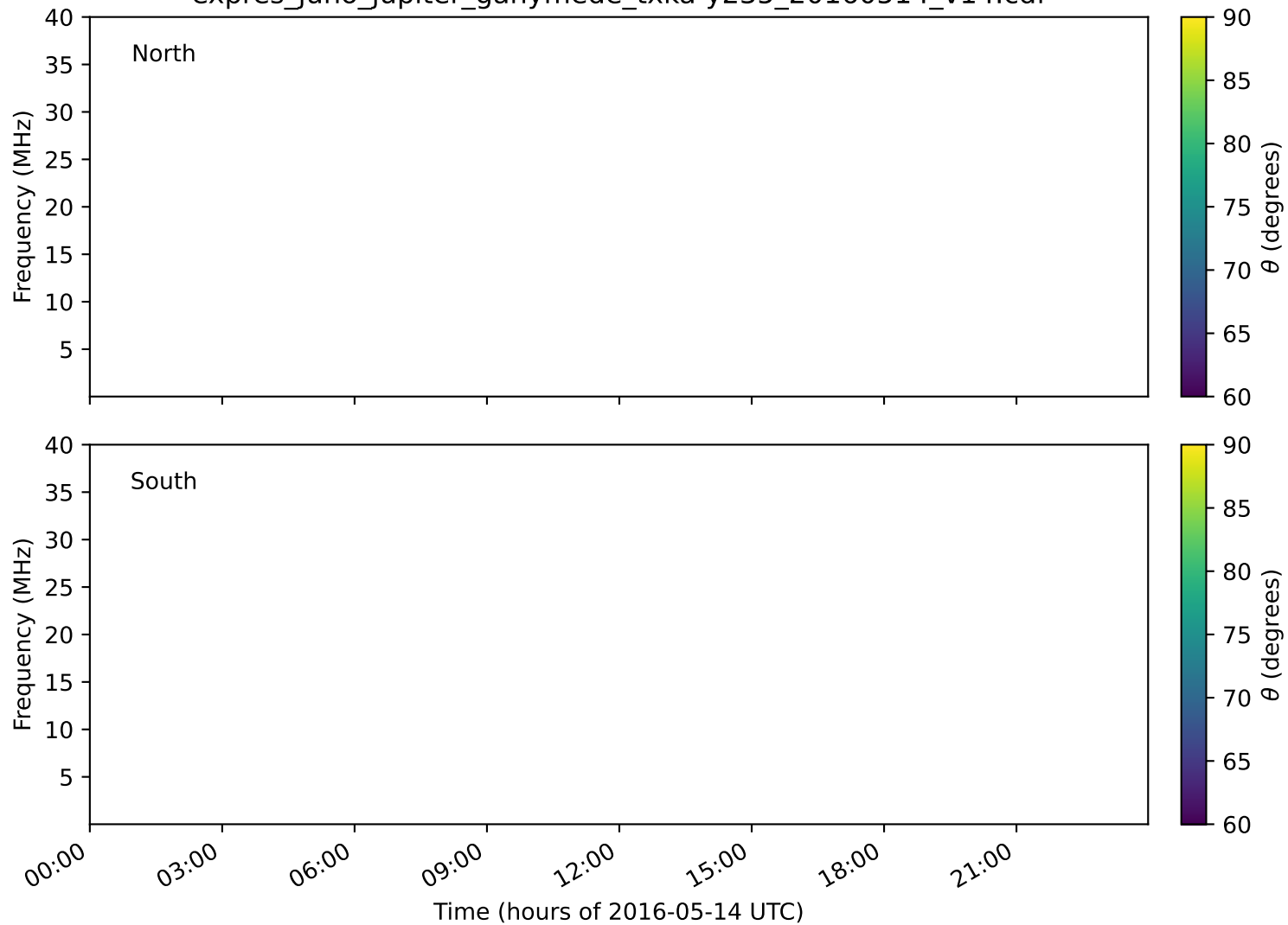
expres_juno_jupiter_ganymede_txka-y235_20160514_v14.cdf
