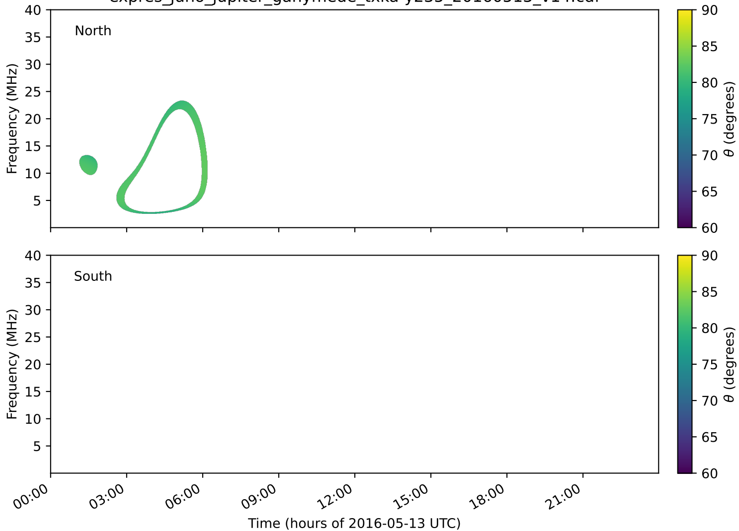
expres_juno_jupiter_ganymede_txka-y235_20160513_v14.cdf
