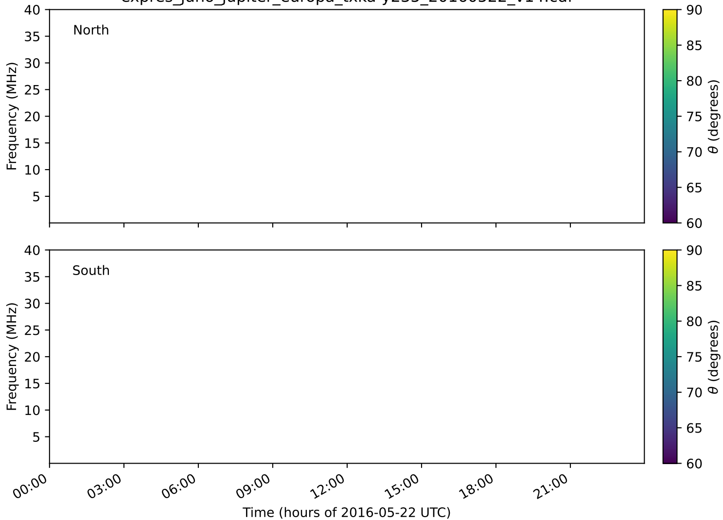
expres_juno_jupiter_europa_txka-y235_20160522_v14.cdf
