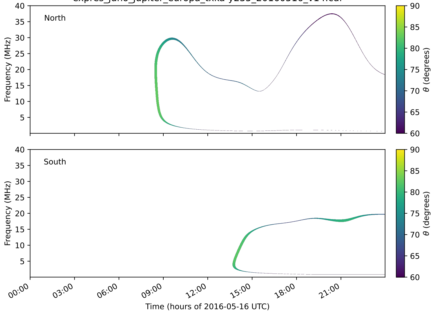
expres_juno_jupiter_europa_txka-y235_20160516_v14.cdf
