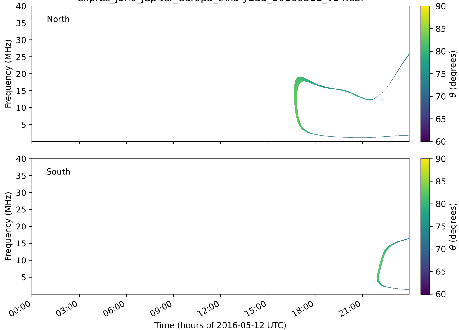
expres_juno_jupiter_europa_txka-y235_20160512_v14.cdf
