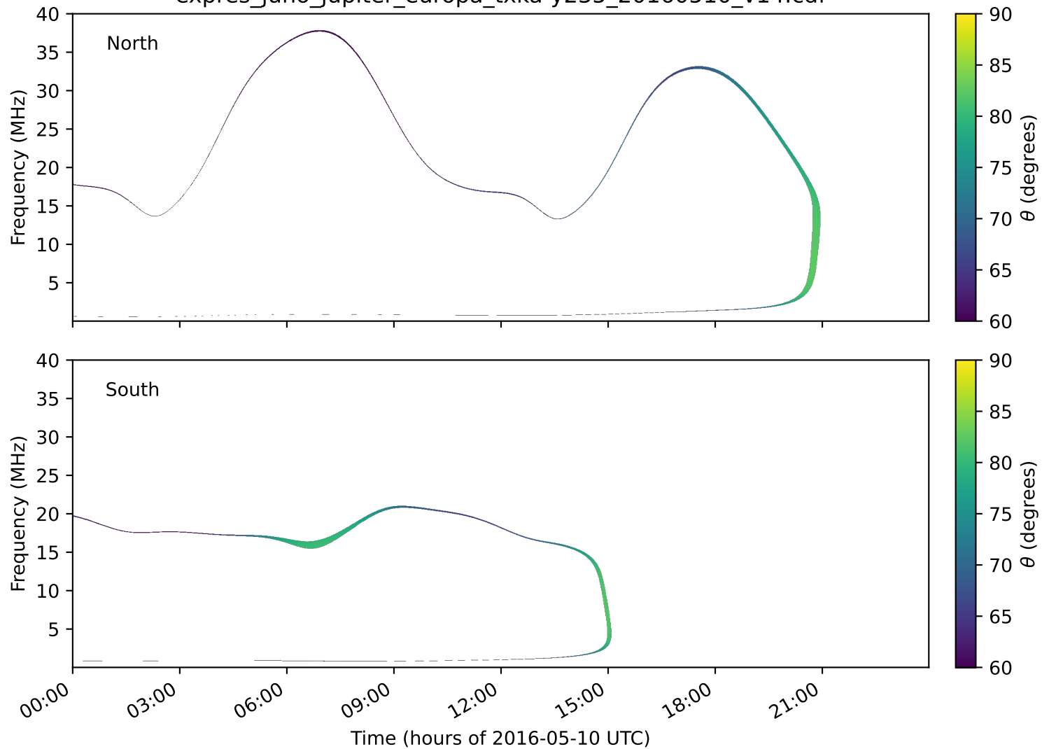
expres_juno_jupiter_europa_txka-y235_20160510_v14.cdf
