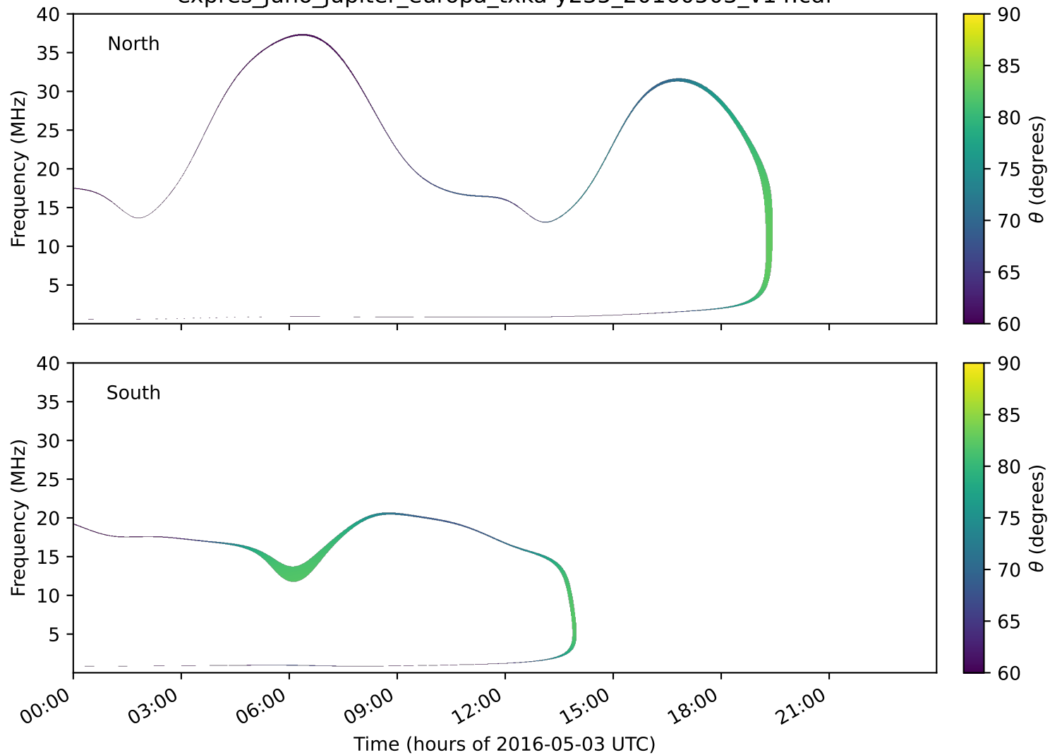
expres_juno_jupiter_europa_txka-y235_20160503_v14.cdf
